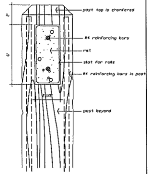
Section thru Rail
