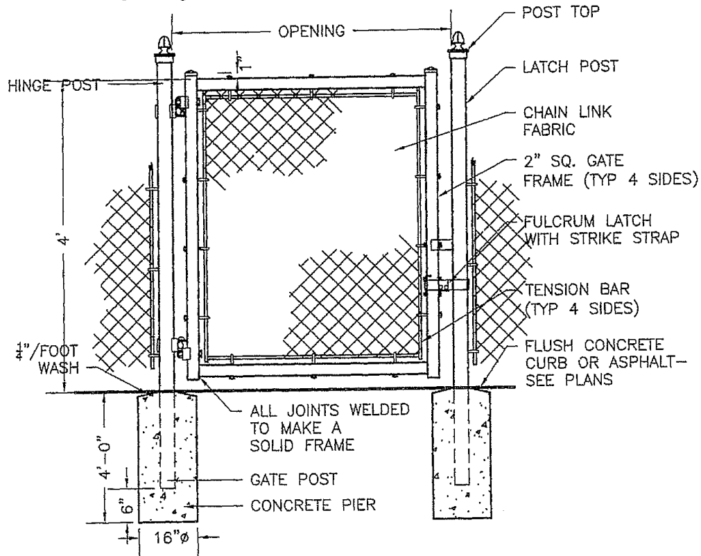
WP -1 (Single Swing Gate Detail)
