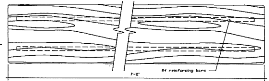
Rail Elevation
