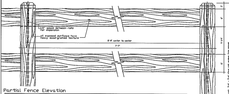
Partial Fence Elevation
