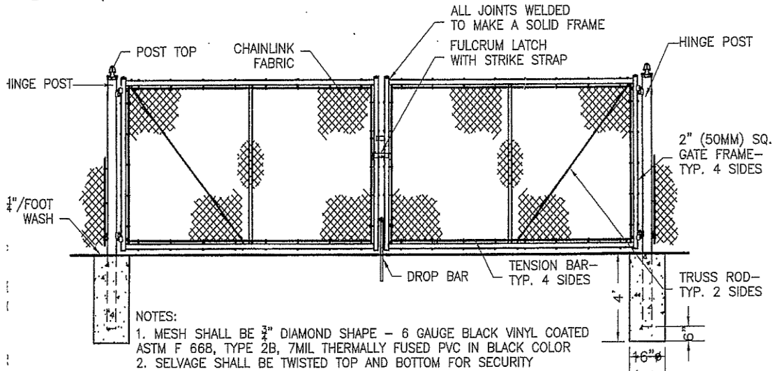
WP -2 (Double Swing Gate Detail)
