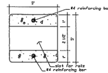
Post Cross Section
